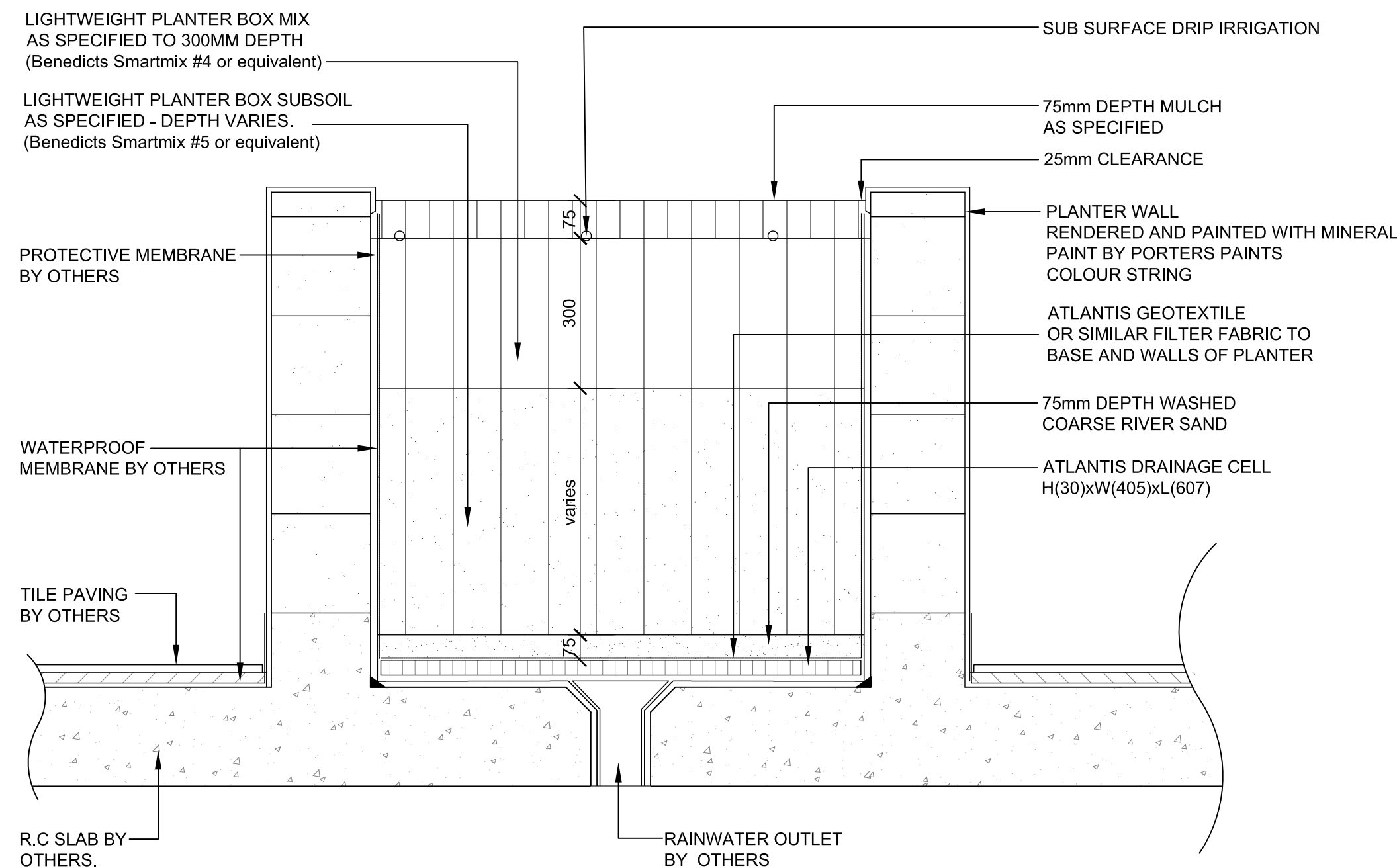
3 PLANTING ON SLAB TYPICAL SECTION 1:10
