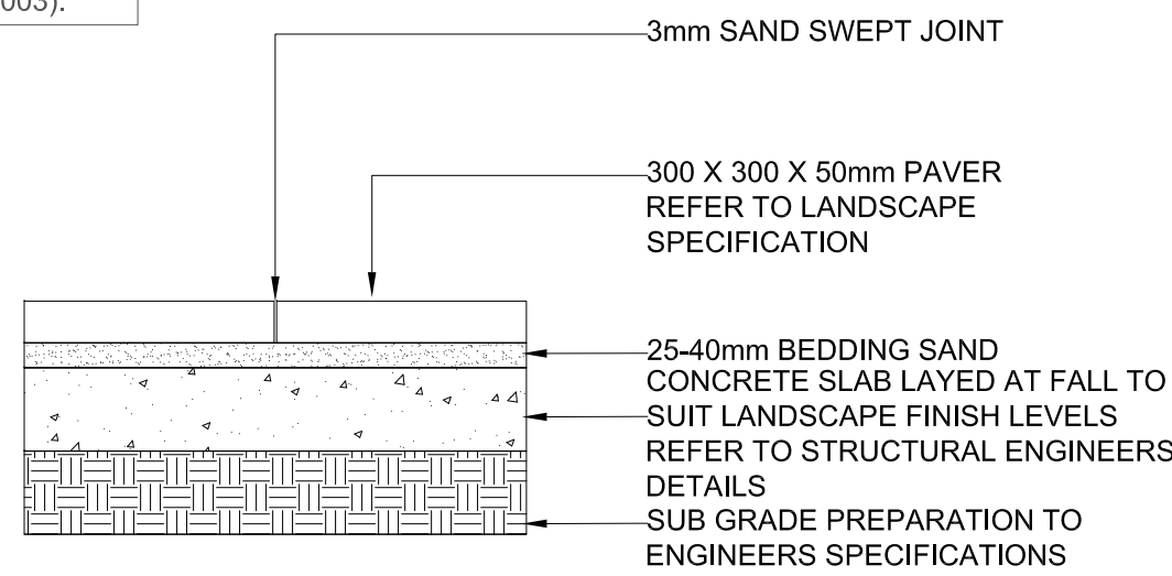
6 PAVING ON CONCRETE SLAB TYPICAL SECTION 1:10
