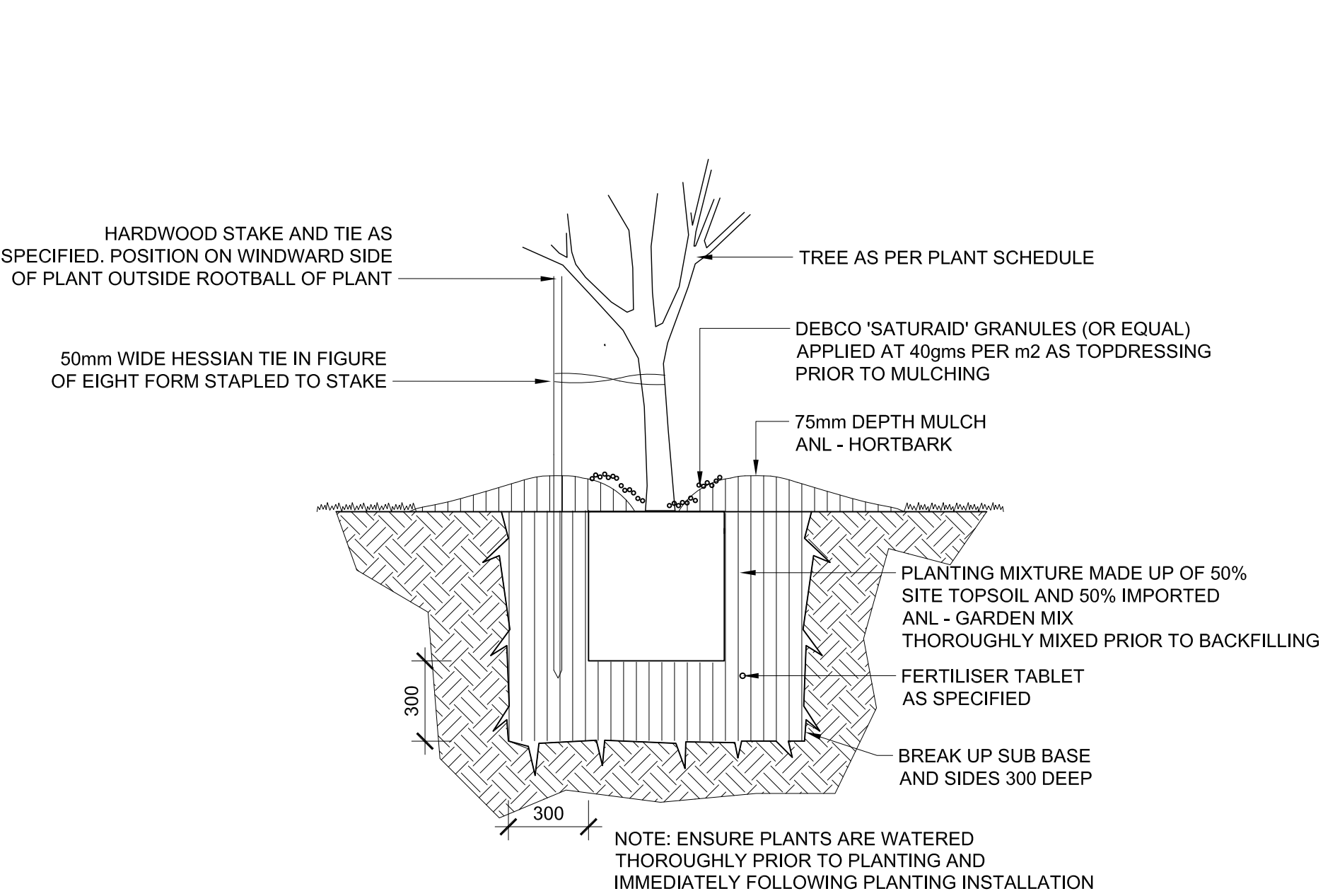
1 TREE PLANTING (75L) TYPICAL SECTION 1:20
