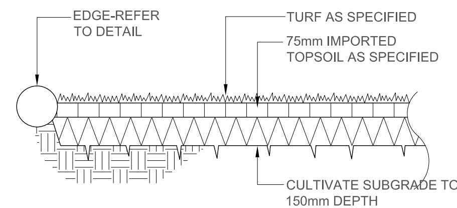
7 TURF ON GRADE SECTION 1:20
