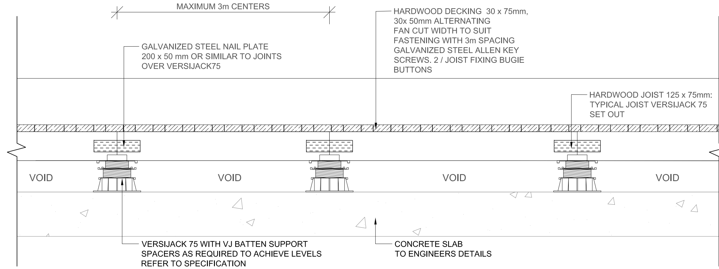
5 TIMBER DECK TYPICAL SIDE ELEVATION / SECTION 1:10
